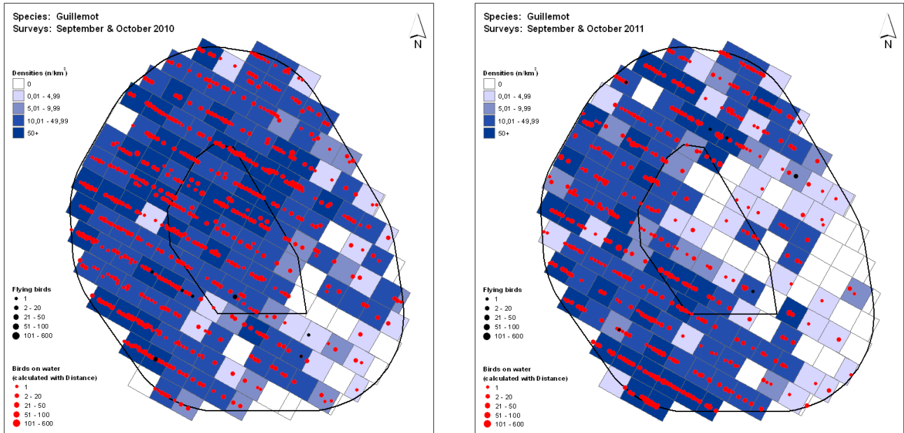
Figure 2. Guillemot density in the Neart na Gaoithe Study Area in September and October, Years 1 and 2.
