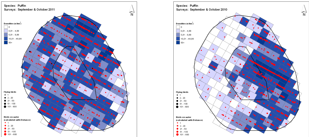
Figure 3. Puffin density in the Neart na Gaoithe Study Area in September and October, Years 1 and 2.
