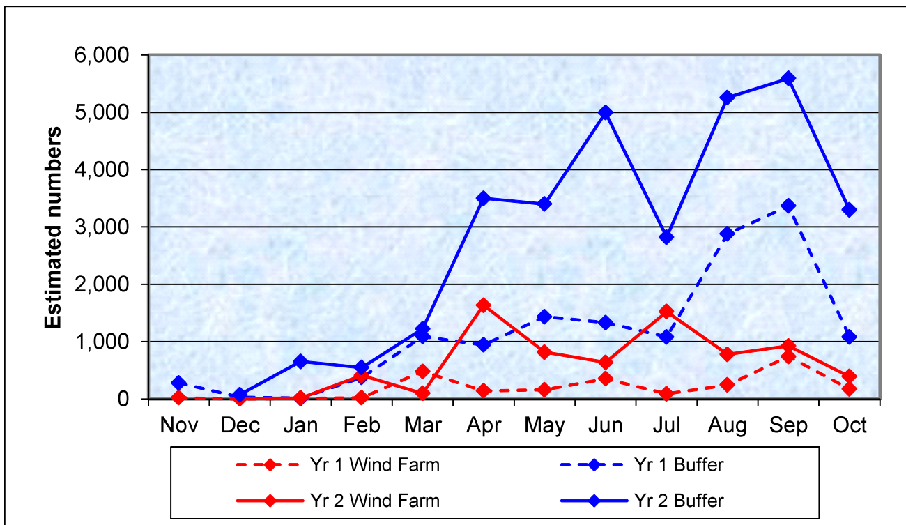
Figure 1. Monthly estimated Gannet population of Neart na Gaoithe Development & Buffer Areas in Years 1 and 2.
